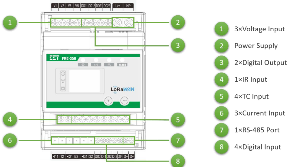
Figure 2-2 Terminals Diagram
