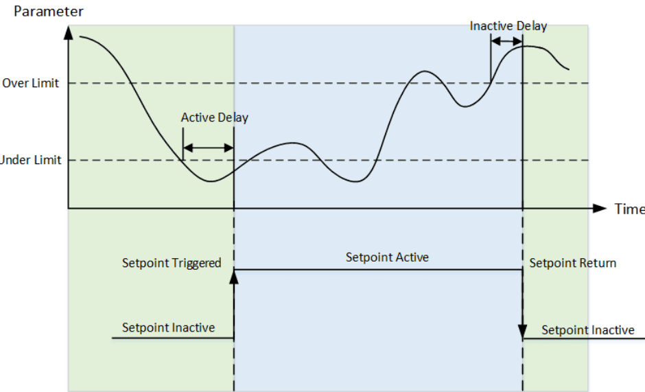
Figure 4-2 Under Setpoint
