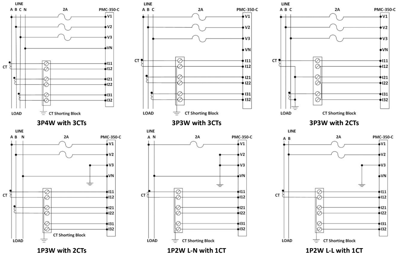
Figure 2-13 Wiring Mode
