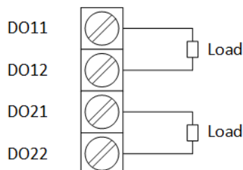
Figure 2-18 DO Connections
