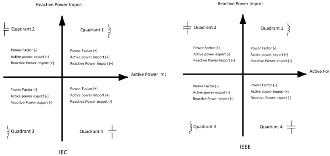
Figure 3-4 PF Convention
