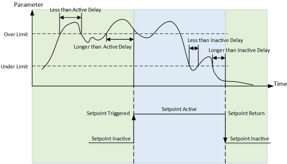
Figure 4-1 Over Setpoint
