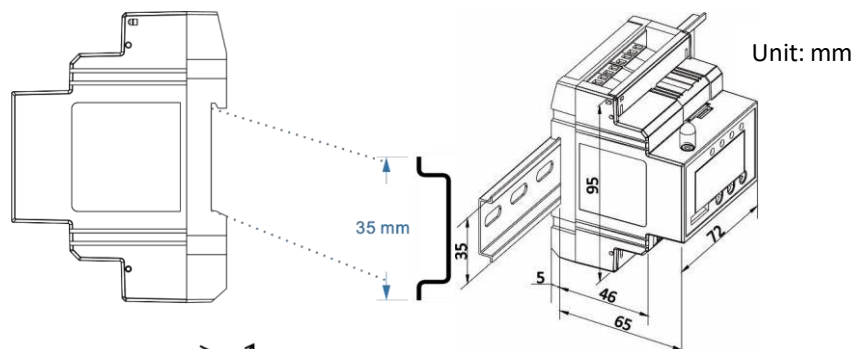
Figure 2-11 DIN-Rail Installation
