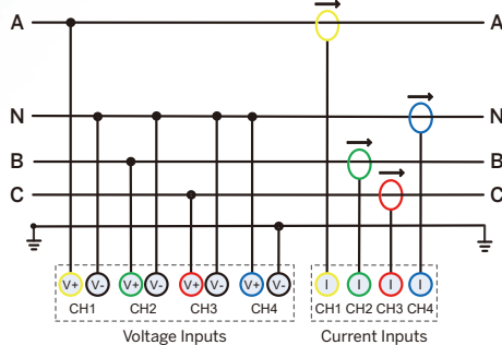
Fig. 1 Wiring Configurations
