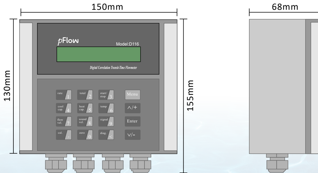
Transmitter
