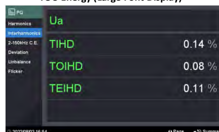
Voltage Interharmonics (Large Font Display)
