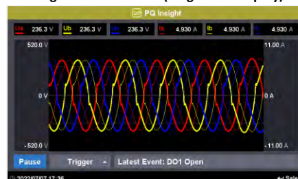
Real-Time Waveform
