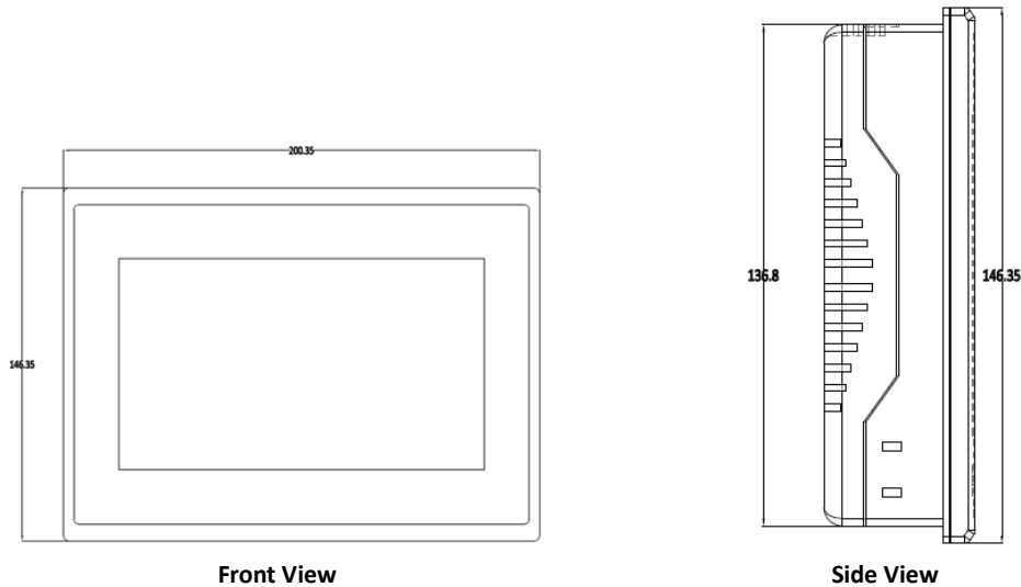
Figure 2-4 HMI Dimensions
