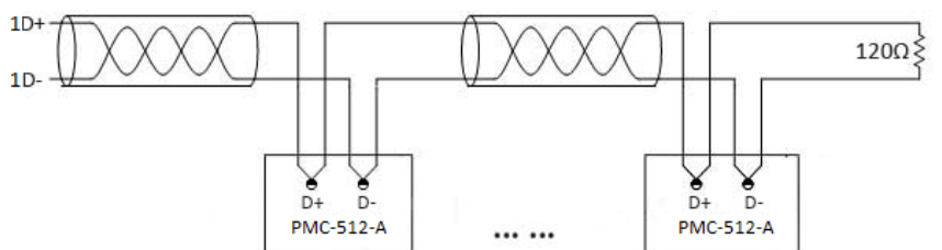
Figure 2-29 Communications Wiring
