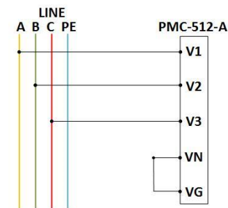
Figure 2-20 3P3W without PTs
