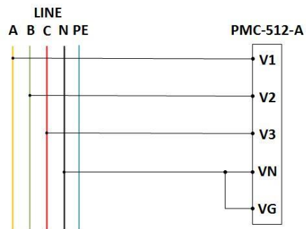
Figure 2-23 3P4W without PTs & VG
