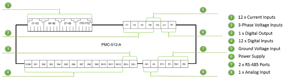
Figure 2-2 Terminal Diagram
