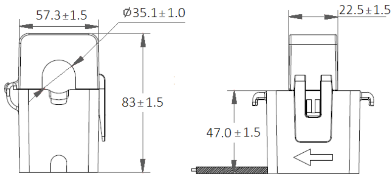
Figure 2-15 PMC-SCCT-400A-40mA-35-A Dimensions
