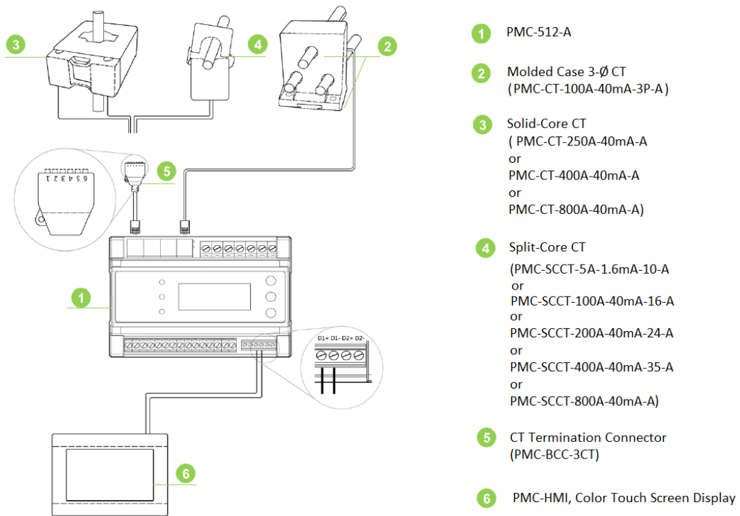
Figure 2-5 Overall Setup
