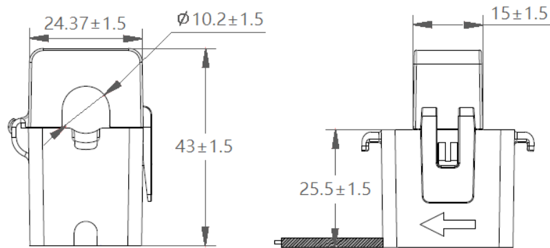
Figure 2-12 PMC-SCCT-5A-1.667mA-10-A Dimensions
