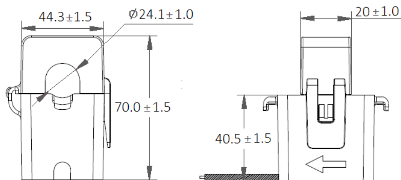
Figure 2-14 PMC-SCCT-200A-40mA-24-A Dimensions
