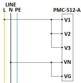
Figure 2-19 1P2W without VG
