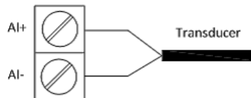
Figure 2-31 AI Wiring
