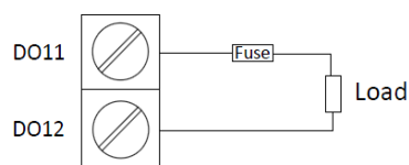
Figure 2-32 DO Wiring
