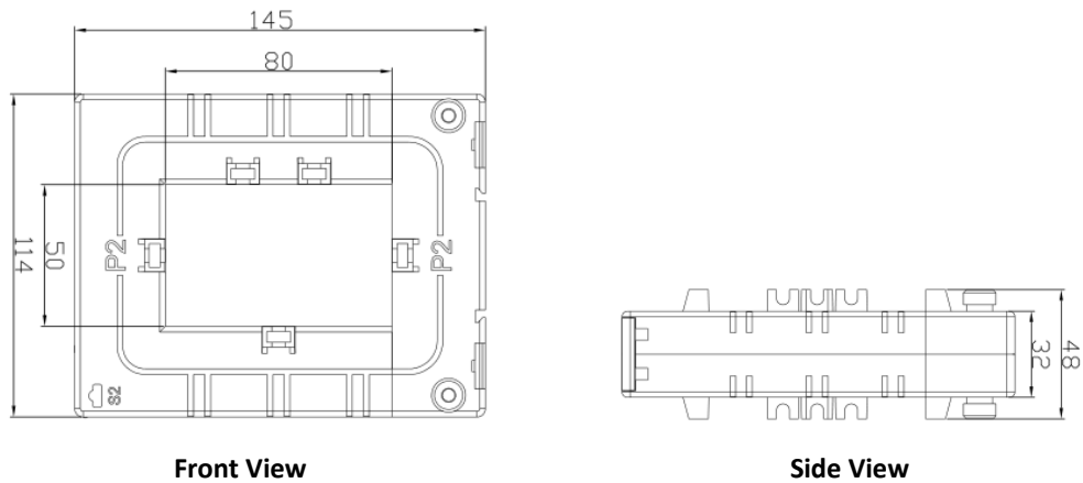
Figure 2-16 PMC-SCCT-800A-40mA-A Dimensions
