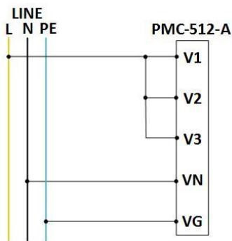
Figure 2-18 1P2W with VG
