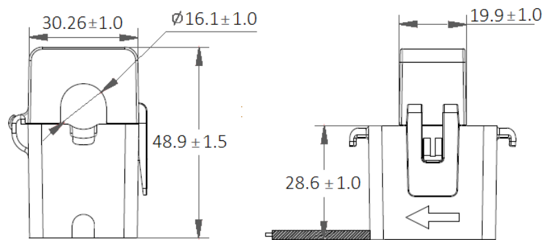
Figure 2-13 PMC-SCCT-100A-40mA-16-A Dimensions
