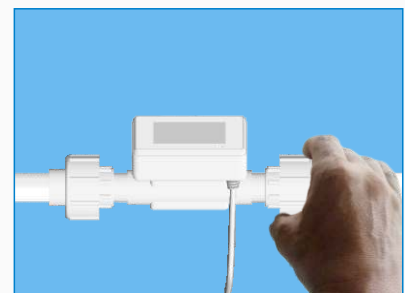
C: Tightening the nuts, and linking the power
