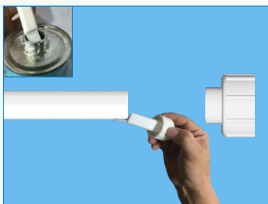
B: Gluing the pipe, and inserting the glued pipe to the joint
