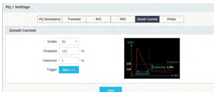
Figure 3-127 Inrush Current Setup Interface
