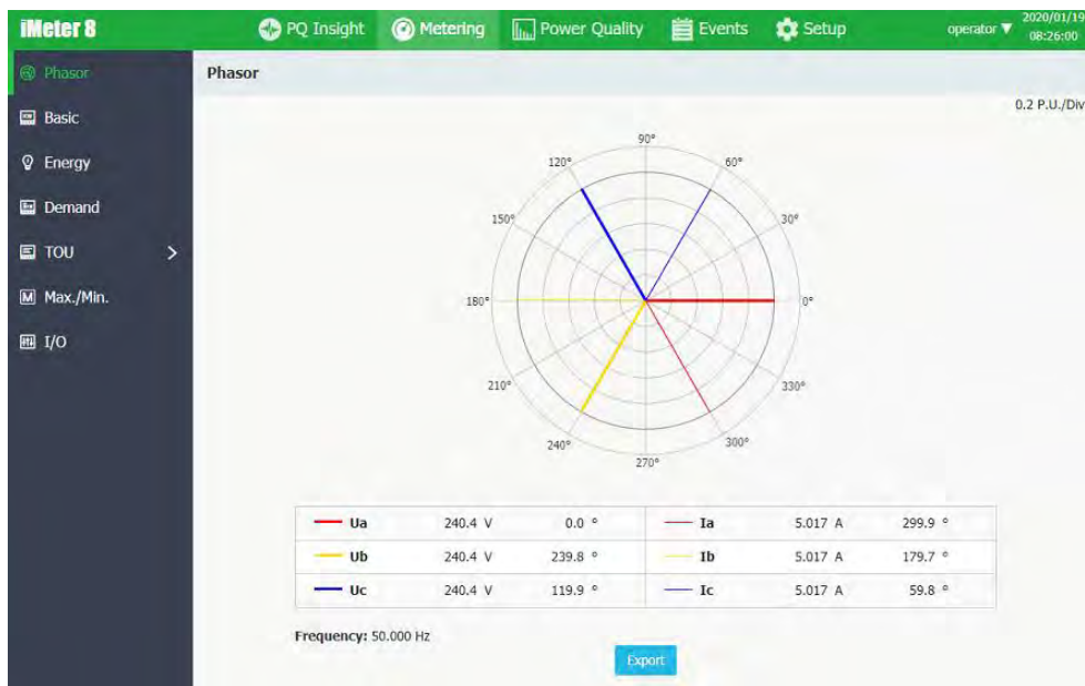
Figure 3-68 Phasor Interface
