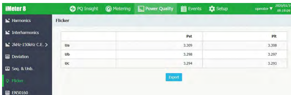
Figure 3-89 Flicker Interfaces
