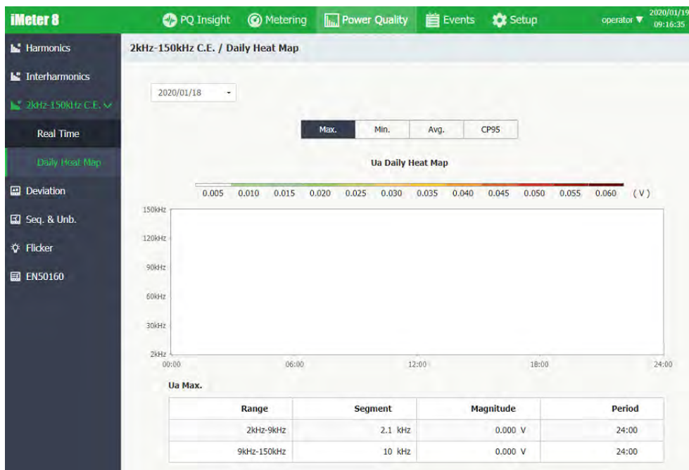
Figure 3-86 Daily Heat Map Interface
