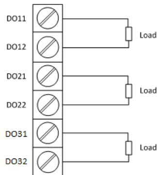
Figure 2-15 DO Connections
