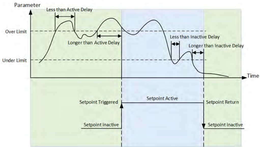
Figure 4-3 Over Setpoints
