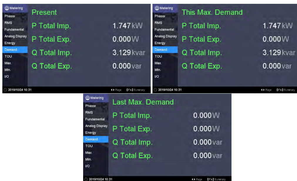
Figure 3-14 Present and Max. Demand Large Font Displays
