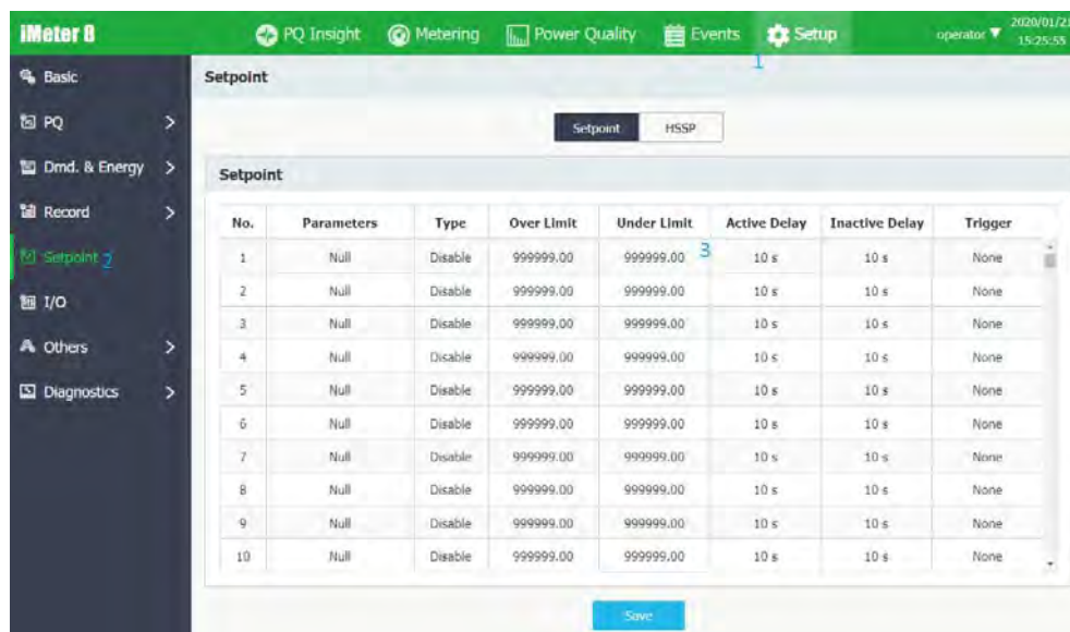
Figure 4-16 Setpoint Settings
