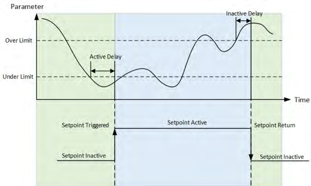
Figure 4-4 Under Setpoints
