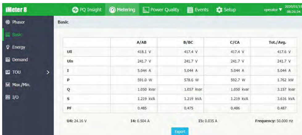
Figure 3-69 Basic Interface
