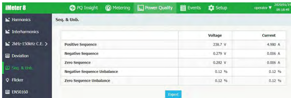
Figure 3-88 Sym. Comp. &amp; Unb. Interface
