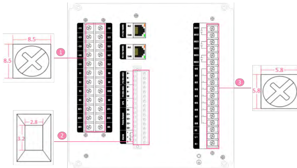
Figure 2-4 Terminal Dimensions
