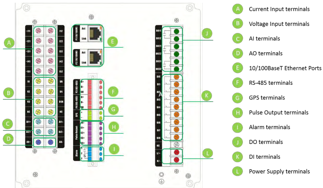
Figure 2-2 Rear Panel
