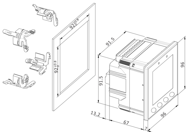
Panel Cutout
